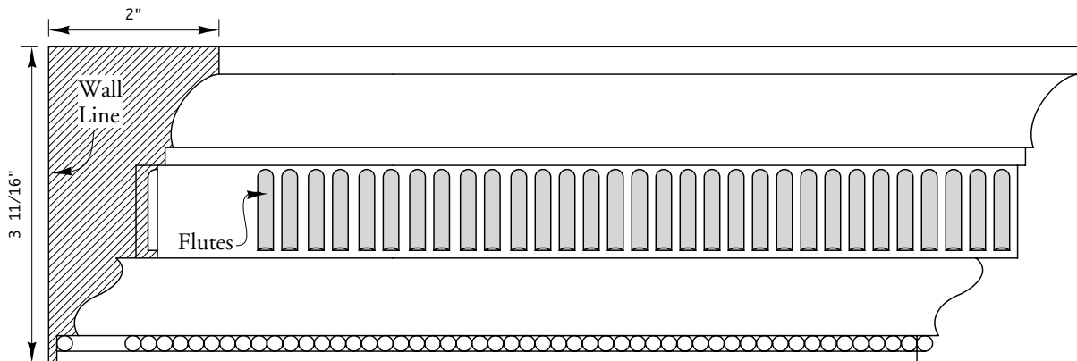
Fig. 37 Shelburne House, London, England, built by Robert Adam 1762-1768, Adam, Works , 1975 reprint, p. 83, vol. II, no. 4, pl. V. 3 \frac{11}{16} \div \text{ratio } .539 = 2" from Wall Line.
